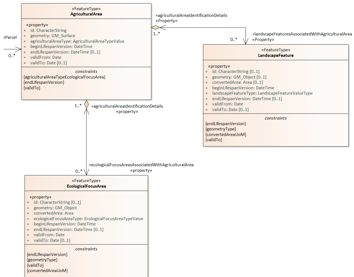
Figure 3. LPIS UML model - AgriculturalArea, LanscapeFeature and EcologicalFocusArea class diagrams and relationships
