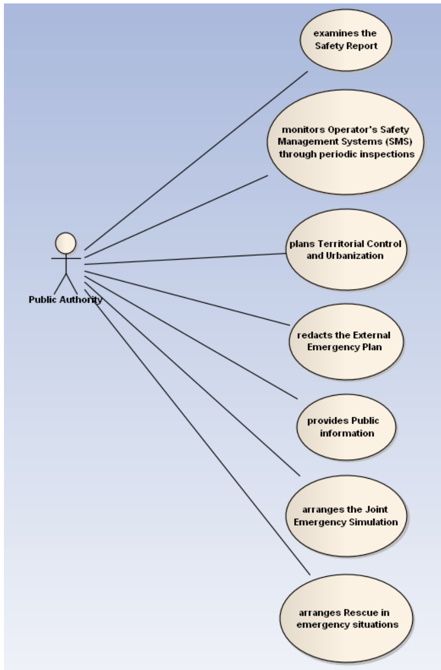
Figure 2 – UML use case diagram, Public authority view
