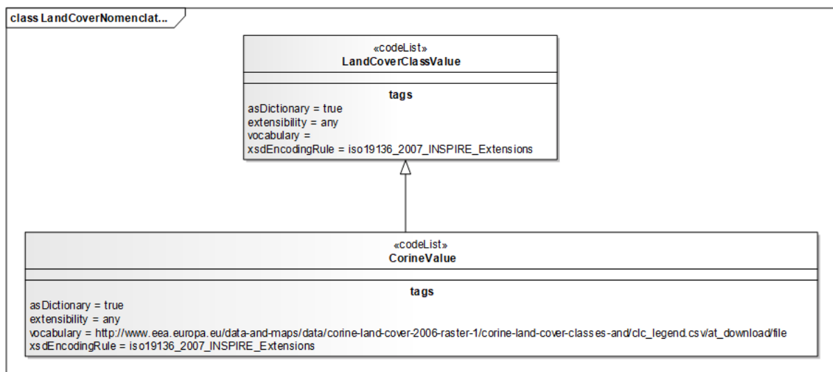
Figure 15 – UML class diagram: CORINEValue
