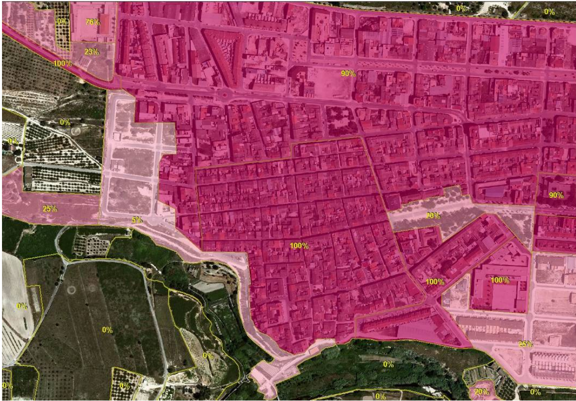
Figure 38: SIOSE polygons of an urban area, indicating the percentage of soil sealed
