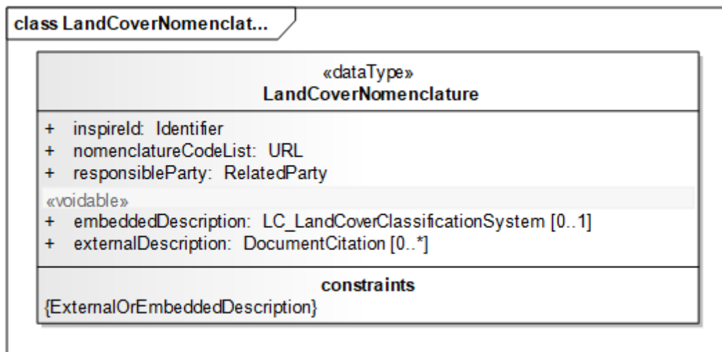
Figure 13 – UML class diagram: LandCoverNomenclature
