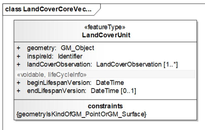
Figure 18 – UML class diagram: LandCoverUnit
