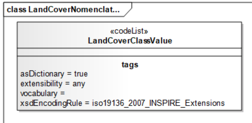
Figure 14 – UML class diagram: LandCoverClassValue
