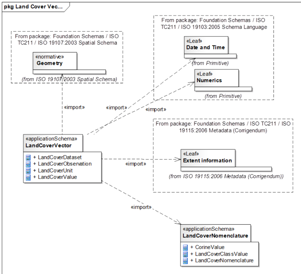
Figure 16 – UML package diagram: LandCoverVector dependencies
