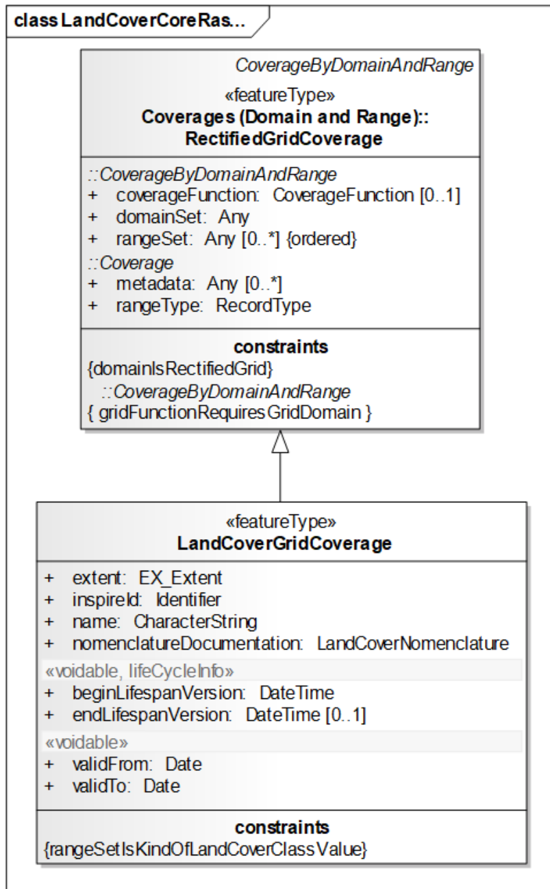
Figure 21 – UML class diagram: LandCoverRaster / LandCoverGridCoverage
