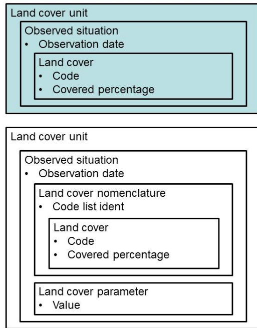
Figure 9 : Land cover description. Core model (top) and extended model (bottom)
