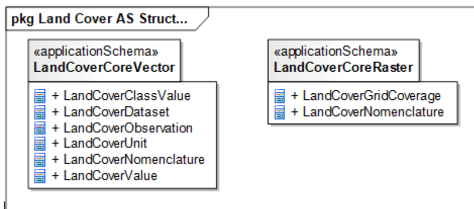
Figure 10 – UML package diagram: Overview of the structure defined for mandatory Land Cover Application Schemas
