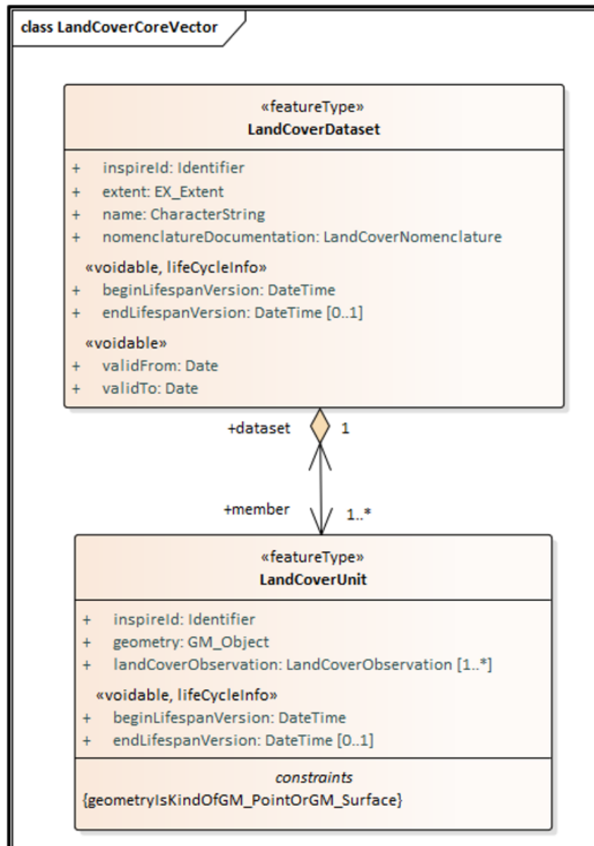
Figure 17 – UML class diagram: Land Cover Data set for vector representations
