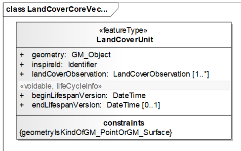
Figure 18 – UML class diagram: LandCoverUnit
