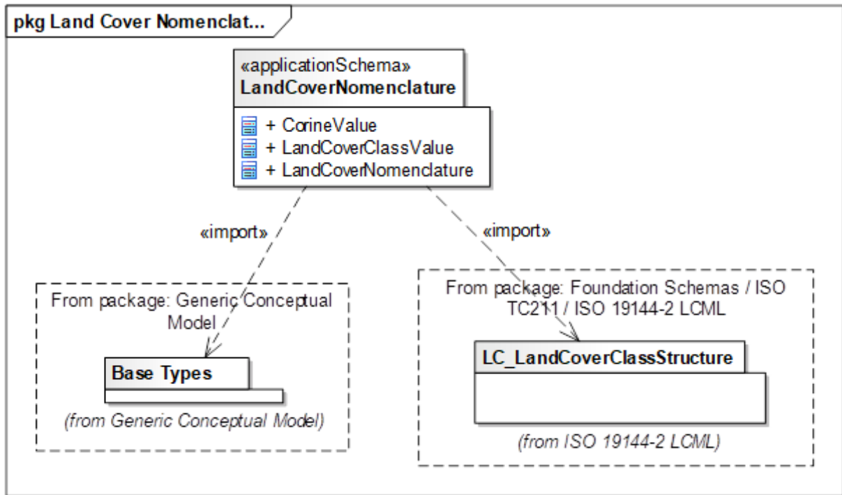
Figure 12 – UML package diagram: LandCoverVector dependencies
