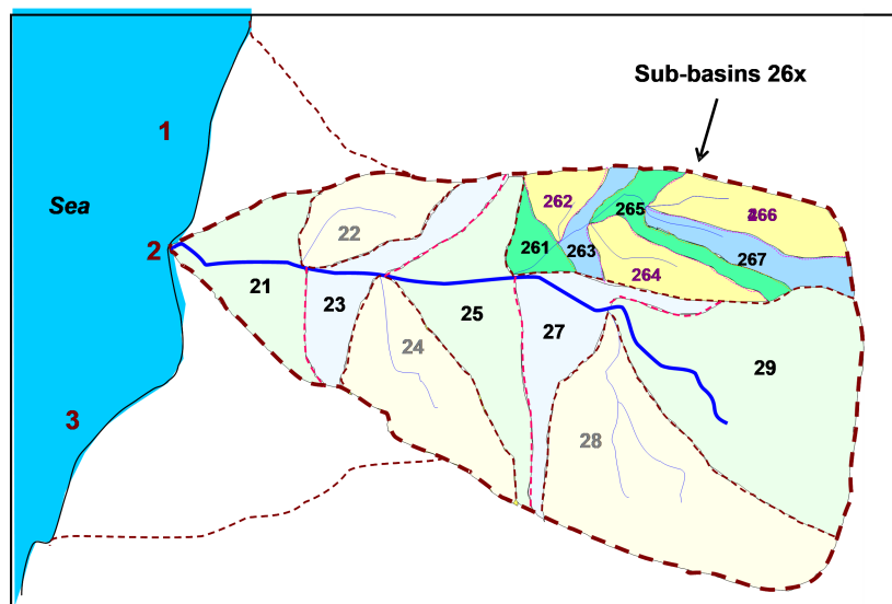
Figure 36 – The Pfafstetter principle of coding drainage-basins and interbasins, illustrated for a hypothetical river basin with code 2. Code 2 indicates the north-eastern primary catchment system within a sea region.
