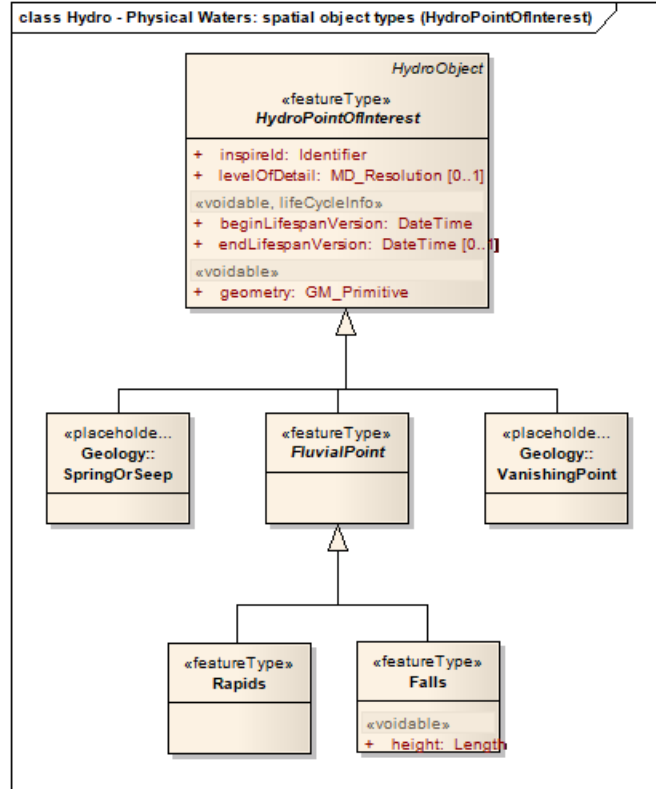
Figure 14 – UML class diagram: 'Physical Waters (HydroPointOfInterest)' spatial object types (including related classes from other themes)
