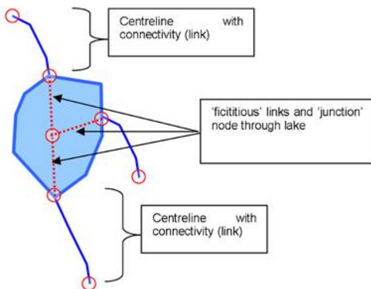
Figure 25 - Links through a lake with multiple inlets / outlets
