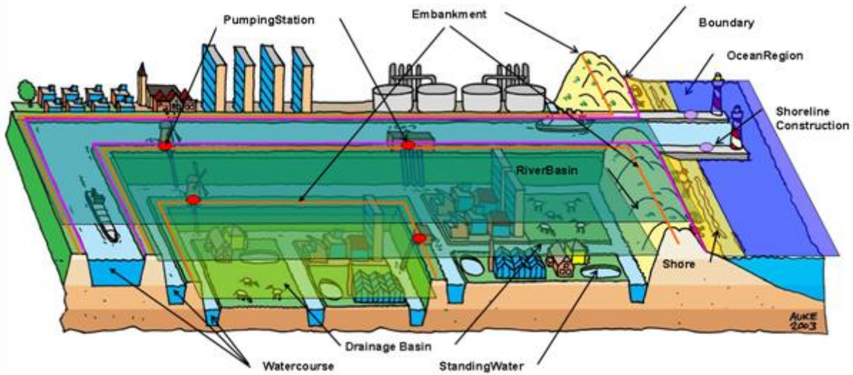
Figure 33 –Modelling of a polder and associated physical waters / related objects
