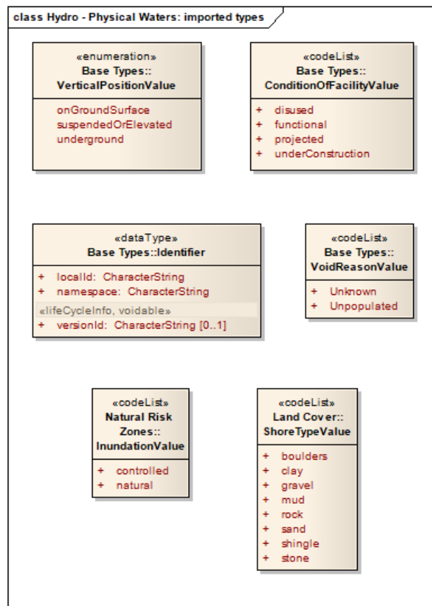
Figure 18 – UML class diagram: 'Physical Waters' additional imported types
