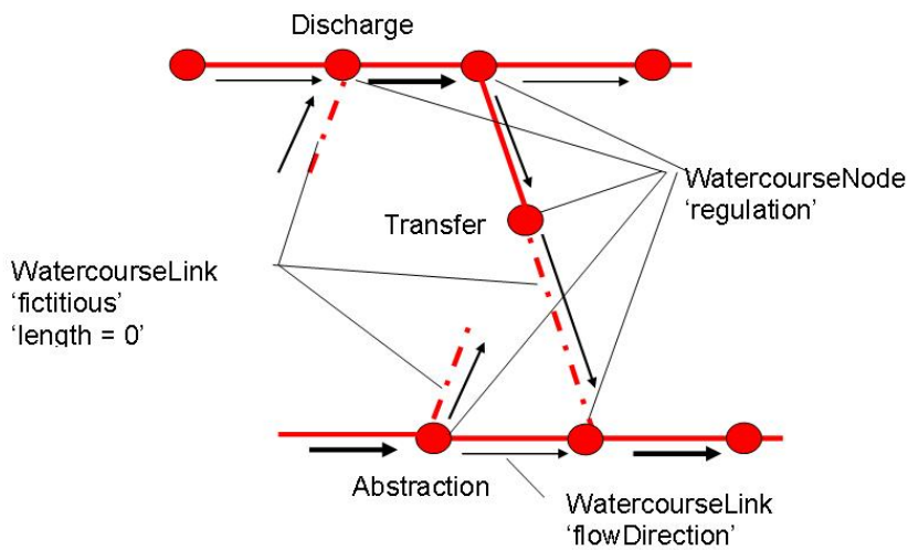
Figure 28 – Modelling of abstraction, discharge and water transfer.
