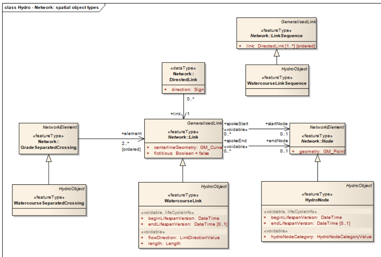
Figure 7 – UML class diagram: 'Hydro – Network' spatial object types
