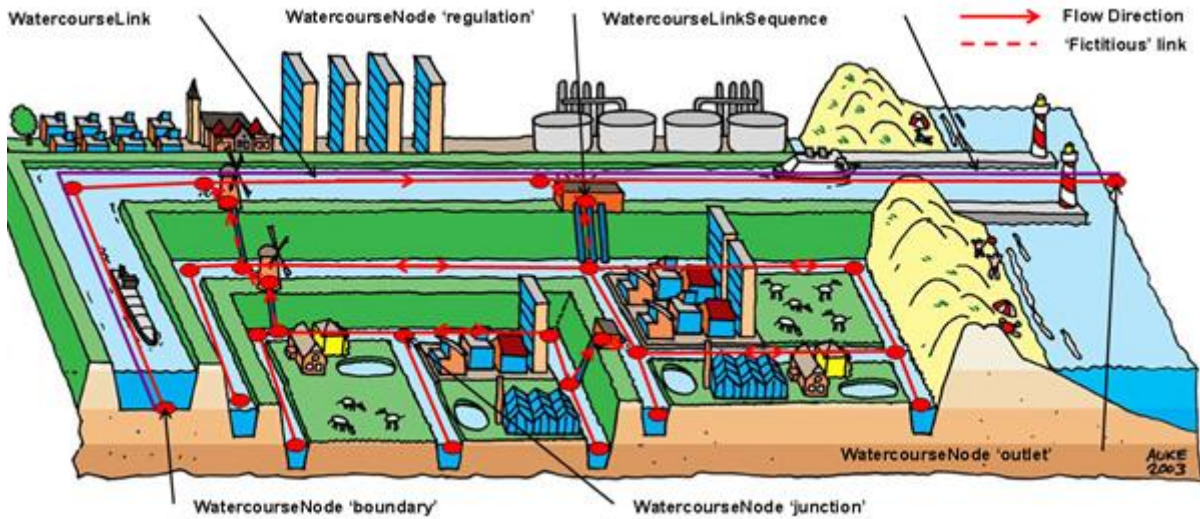
Figure 40 – Network elements in a polder situation
