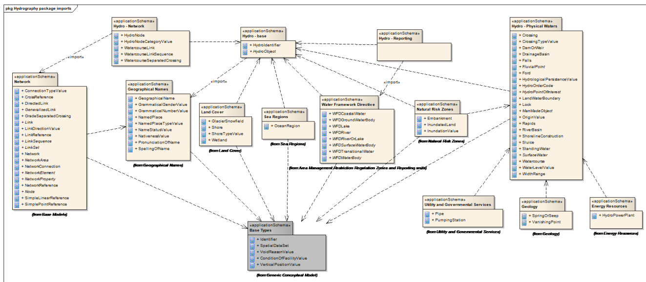
Figure 3 – Package relationships in the Hydrography application schemas
