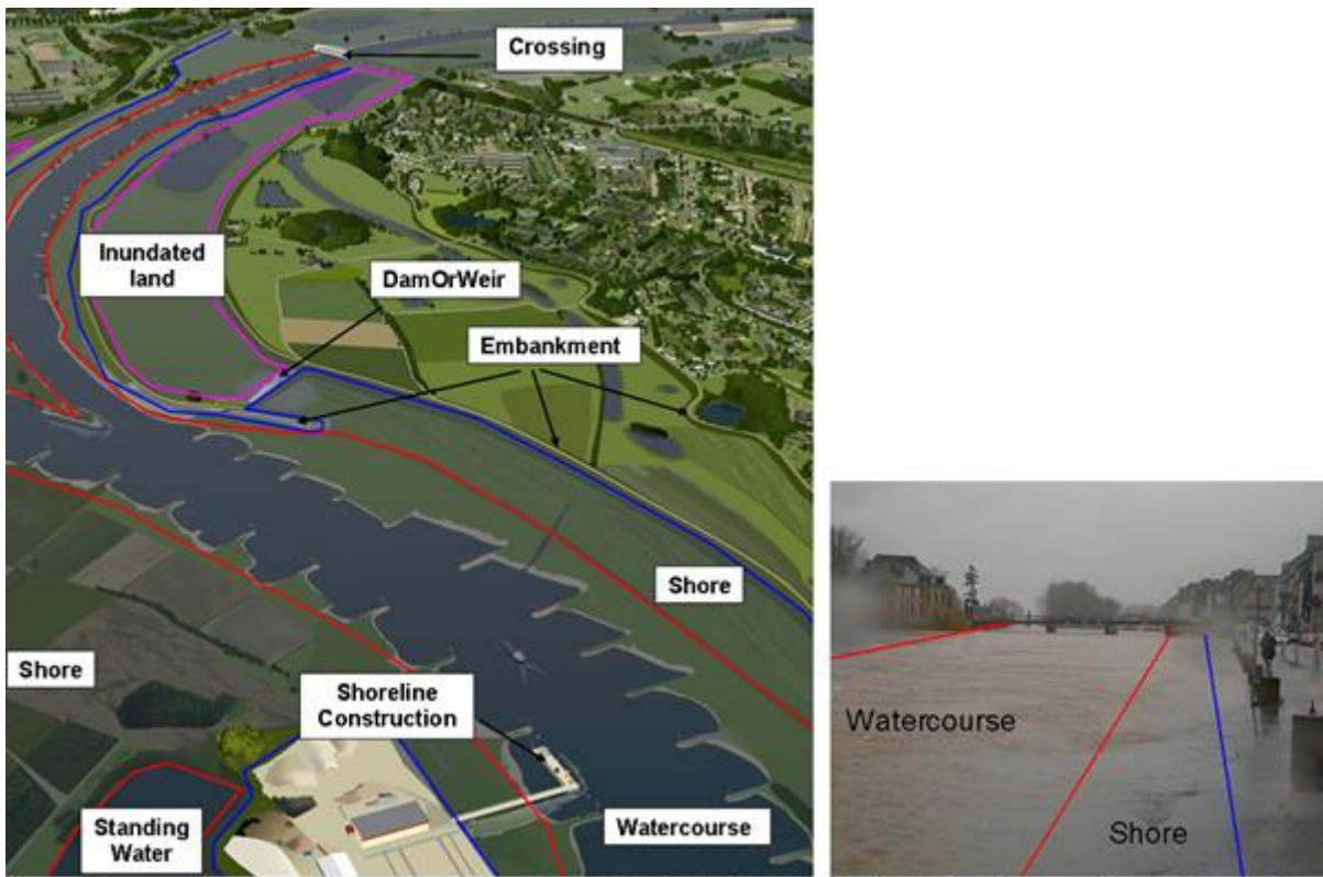
Figure 19 - watercourse, shore and inundated land; in the right situation the overflowed bank is not considered inundated land.
