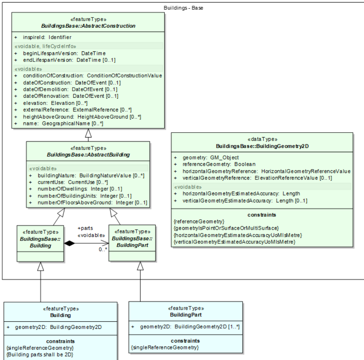
Figure 25: The Buildings 2D application schema
