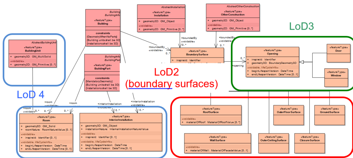
Figure 55: Modeling of LoD2, LoD3 and LoD4
