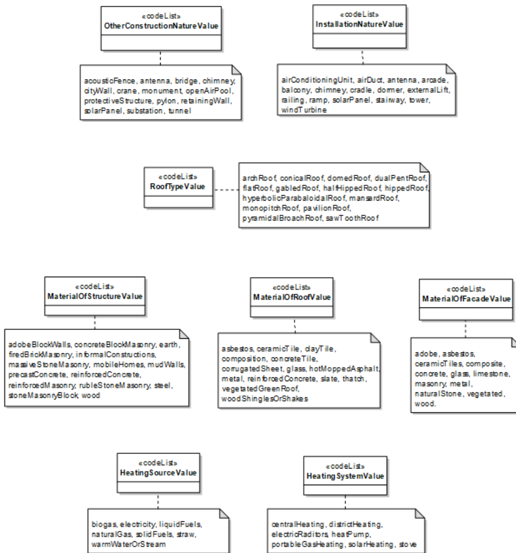
Figure 52: Overview of BuildingExtendedBase - Code lists
