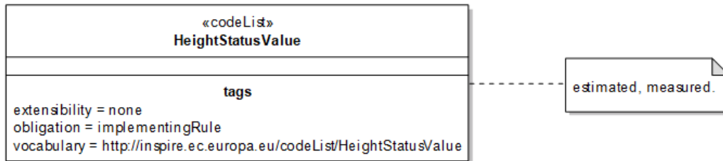
Figure 16: The HeightAboveGround data type
